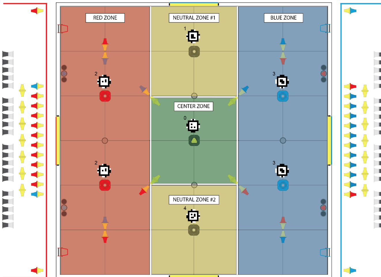
Figure 1.5.2: Achieve Pinnacle field with AprilTag locations and highlighted zones
